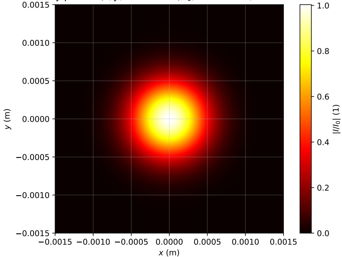
Intensity profile I(x, y, z = 0.080m)/I_0 , P_{in}=0.8P_{cr} , artificial time
